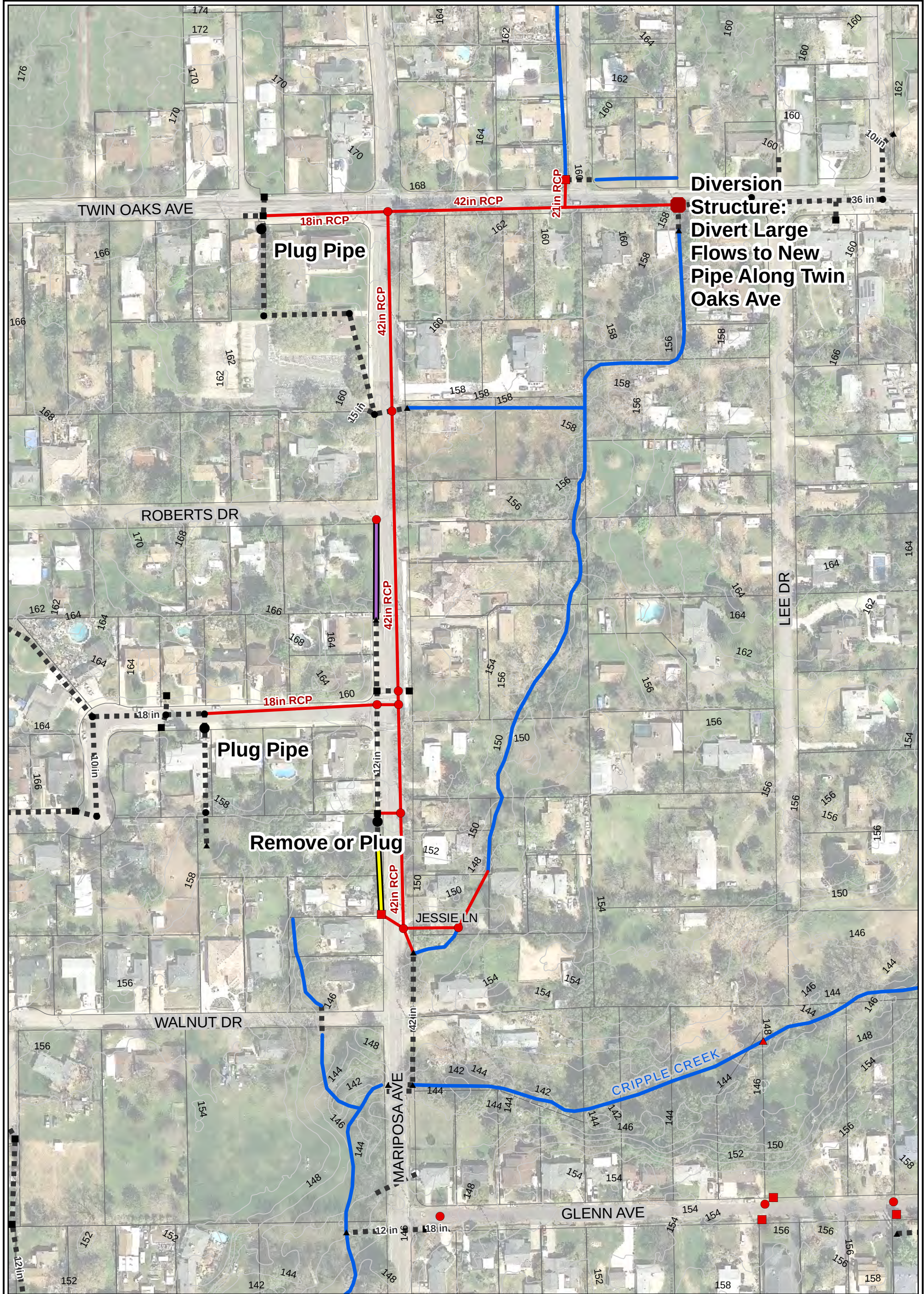
Figure 7-5 City of Citrus Heights Neighborhoods 6 and 7 Drainage Master Plan Study Problem Locations 2, 3, and 11 Proposed Solution
